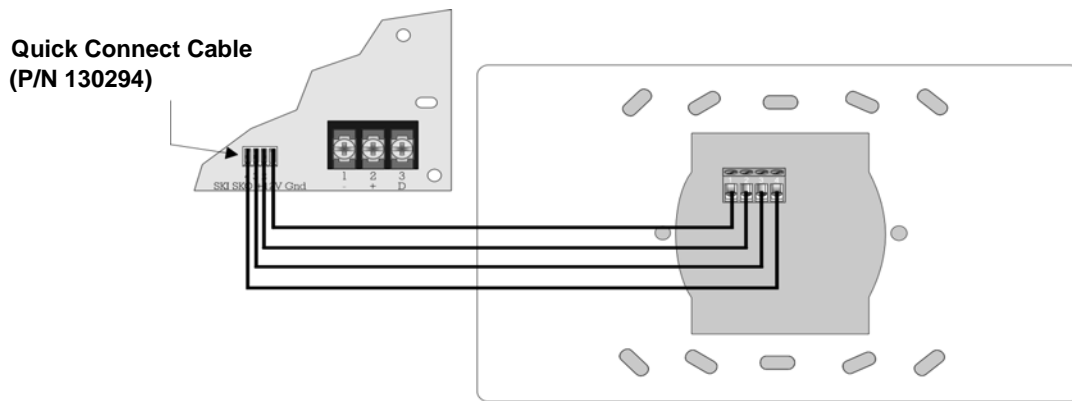
Figure 4-1 5230 Connections to the SK-2104.
